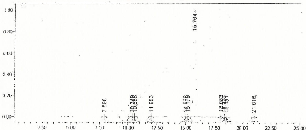
Auto-Scaled Chromatogram
